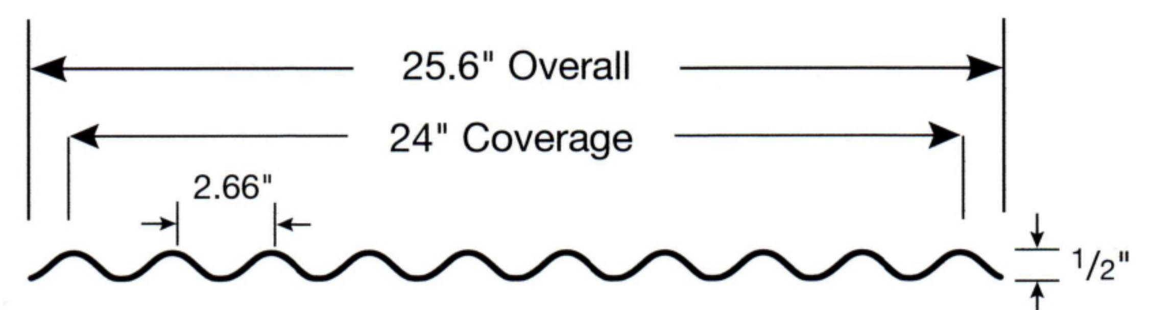
Corrugated Profile
